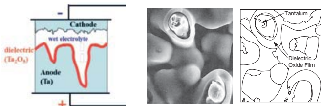
Figure 1 a. Basic Tantalum Wet Electrolytic Capacitor System
