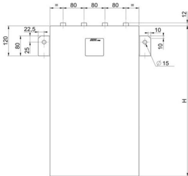
Female terminals
