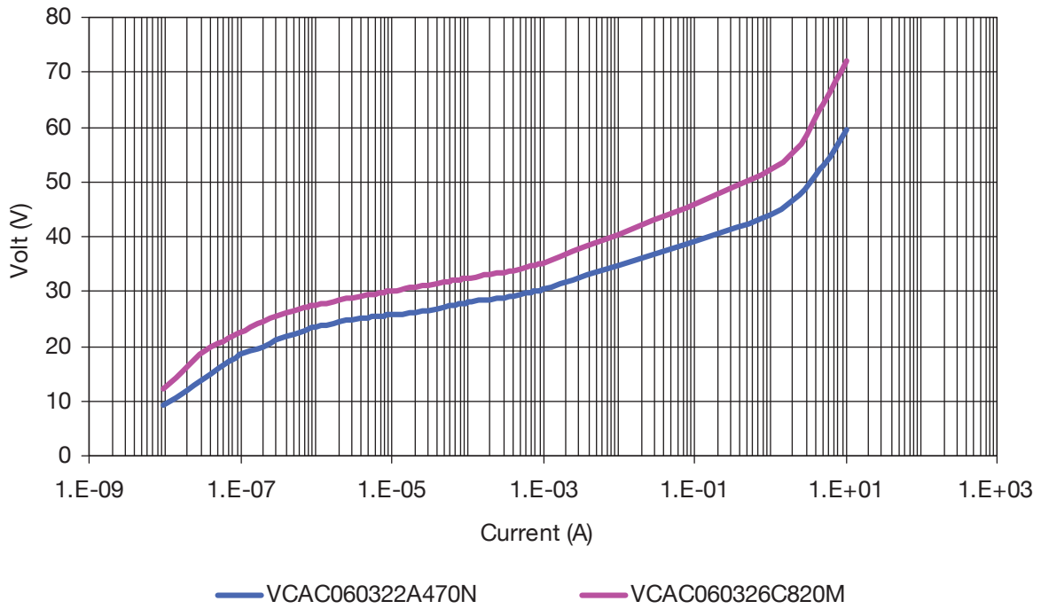
V-I Curve
