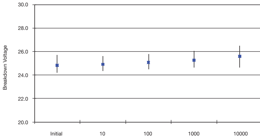
ESD 8 kV IEC 61000-4-2 150pF / 330Ω Resistor VC060318A400
