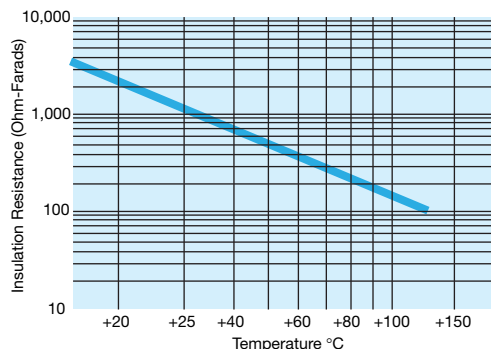
Insulation Resistance vs. Temp.
